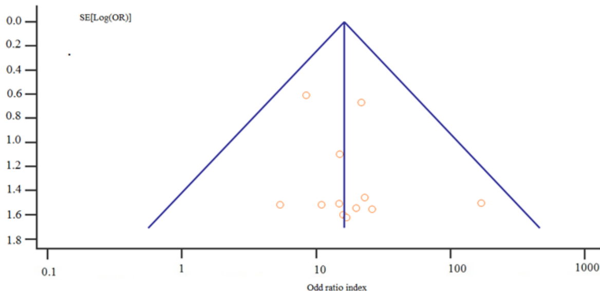
Figure 3. Funnel plot for the evaluating publication bias for the correlation between CDHI methylation and NPC risk
