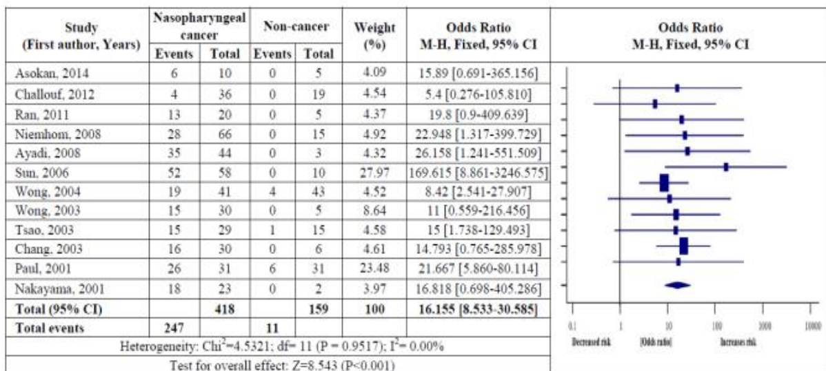
Figure 2. Forest plot of the correlation between CDHI methylation and NPC risk
