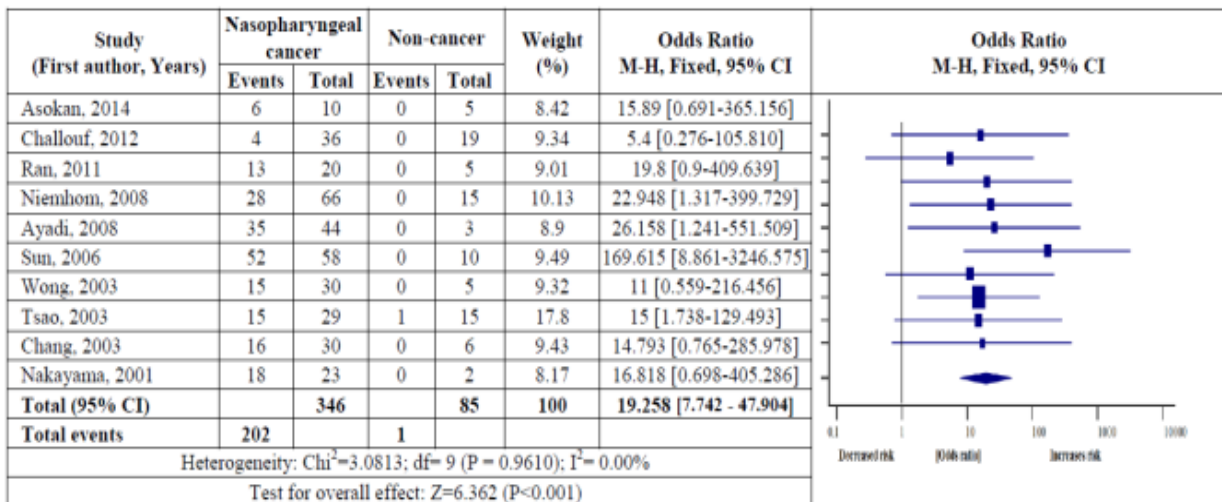
Figure 4. Forest plot of the correlation between CDH1 methylation and NPC risk in Asian
