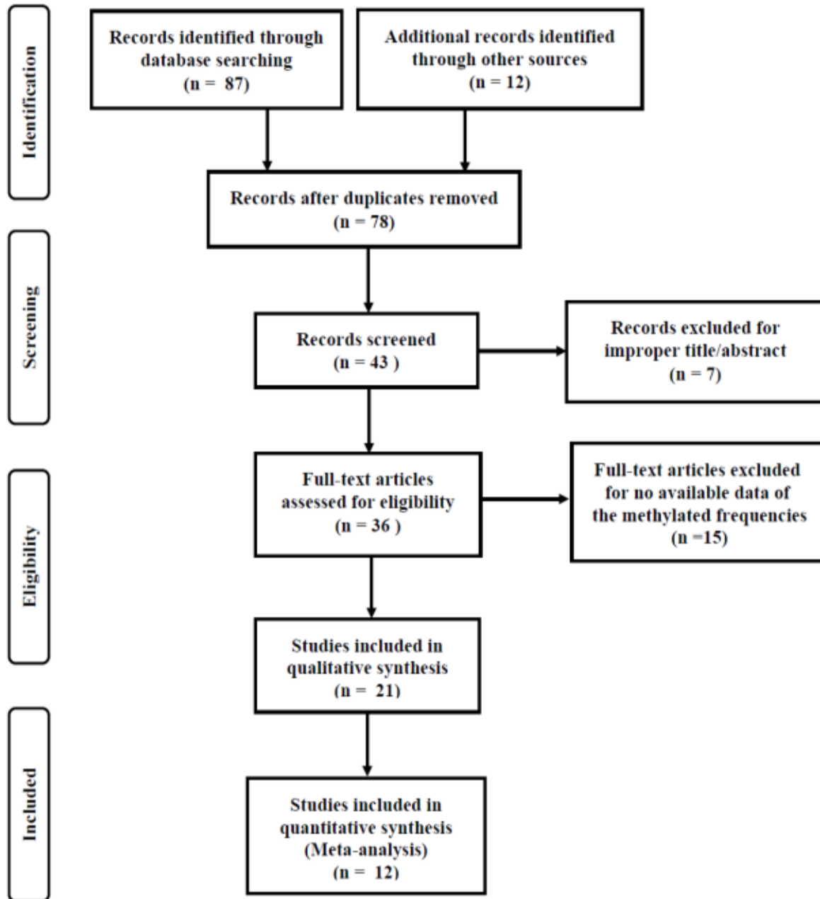
Figure 1. The flow chart of systematic review process
